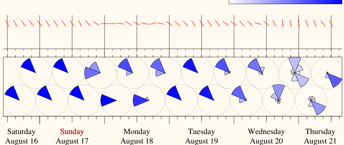
Distribution of 10m Wind Direction
